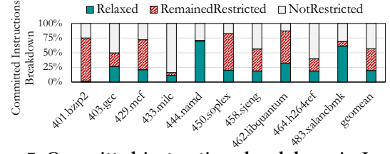
Figure 7: Committed instructions breakdown in LEVIOSO based on their restrictions: (1) Relaxed: restrictions relaxed via compiler information, (2) RemainedRestricted: restrictions remain despite compiler information, (3) NotRestricted: no restrictions. Note, that the instruction counts do not equate to performance.
