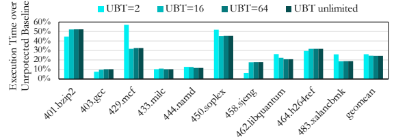
Figure 8: Execution time of LEVIOSO over the Unprotected Baseline with different UBT sizes.
